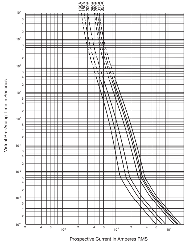
Time-Current Curve
